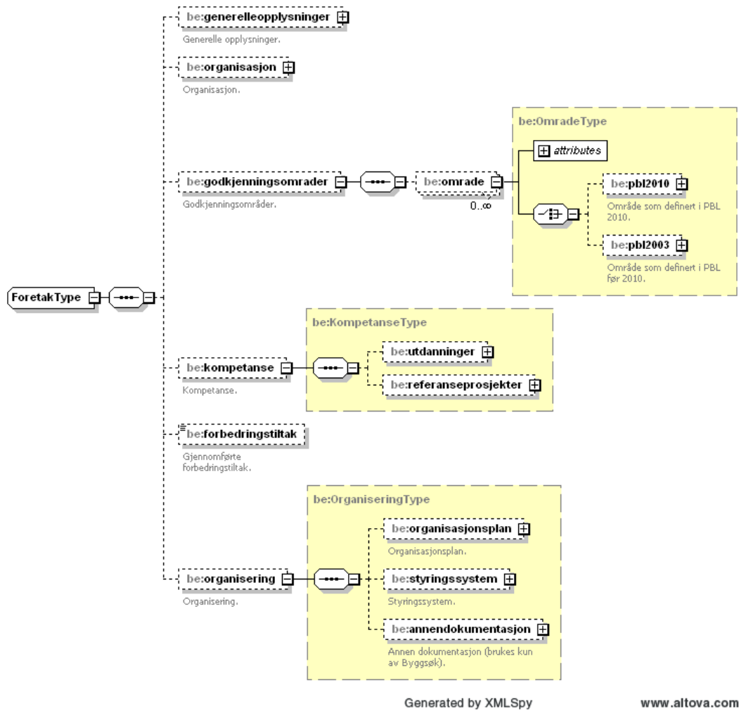
Figure 74 Complex type ForetakType
