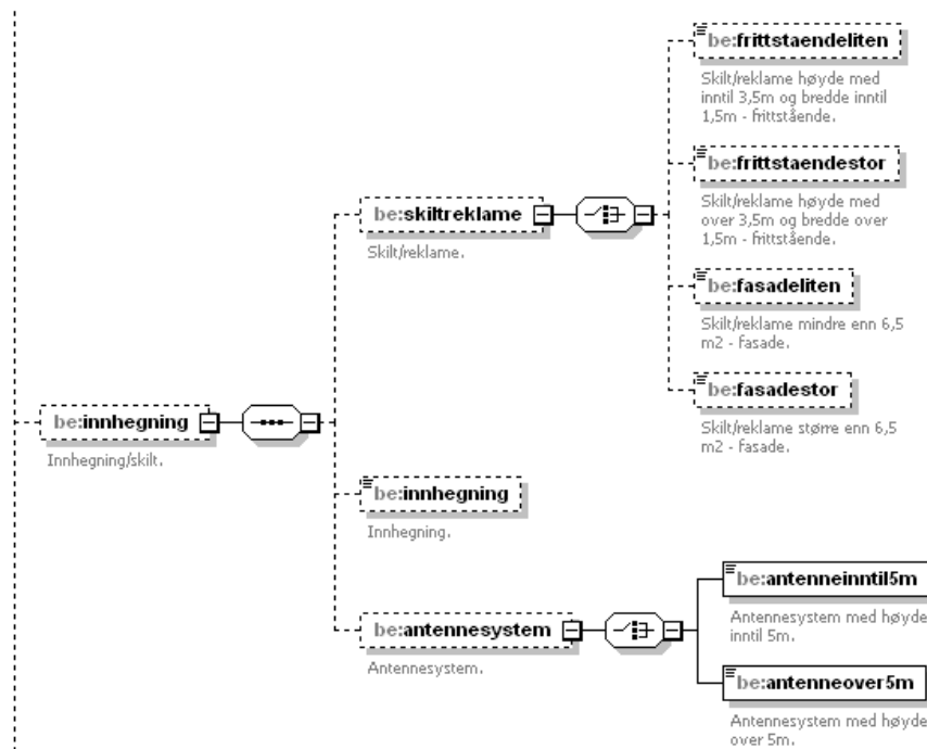
Figure 105 'innhegning' within TiltakType
