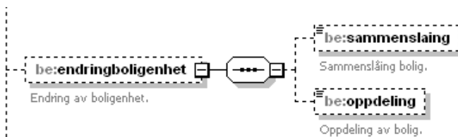
Figure 101 "endringboligenhet" within TiltakType
