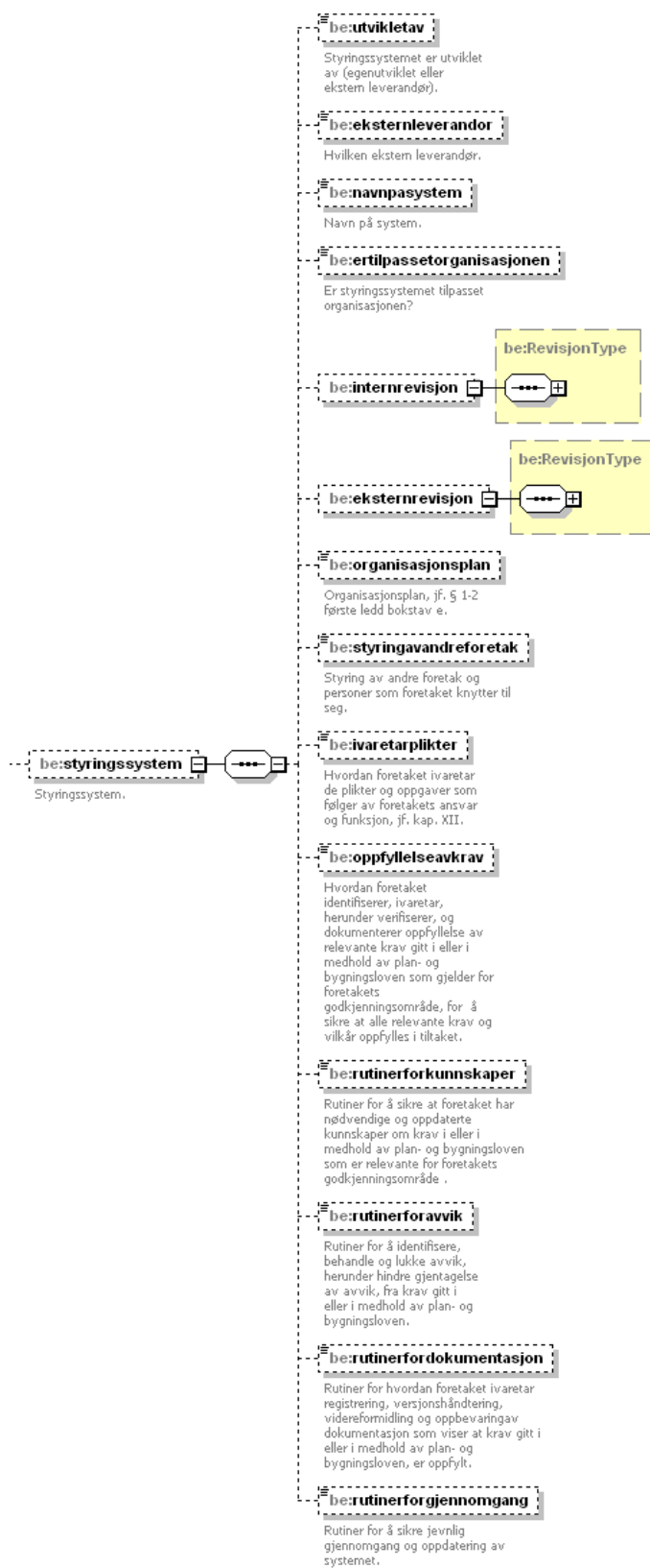
Figure 85 'styringssystem' within OrganiseringType
