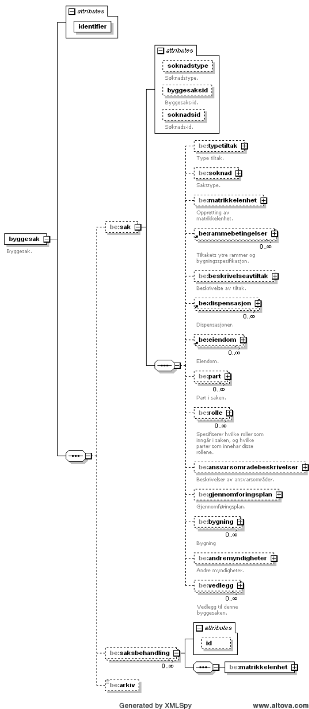
Figure 15 The element structure of 'byggesak'
