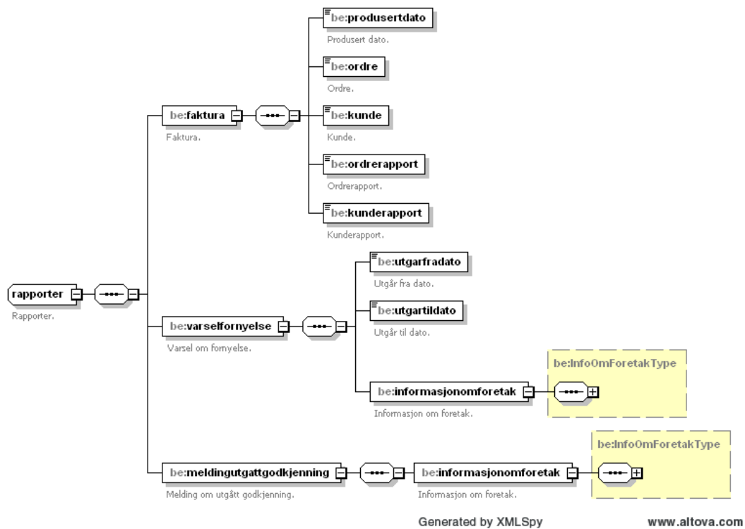
Figure 57 Complex type rapporter
