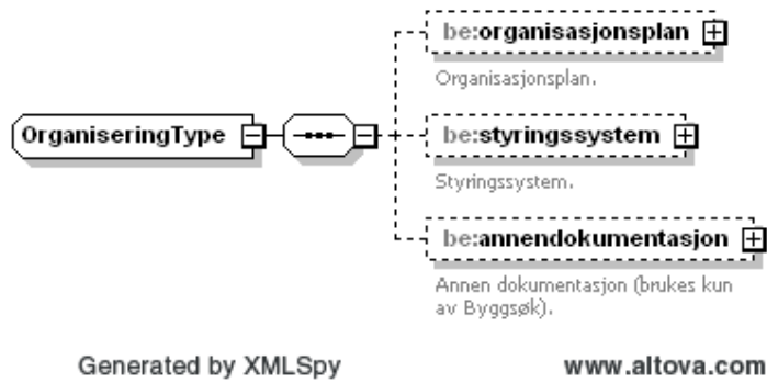
Figure 83 Complex type OrganiseringType
