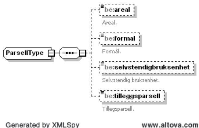
Figure 87 Complex type ParsellType
