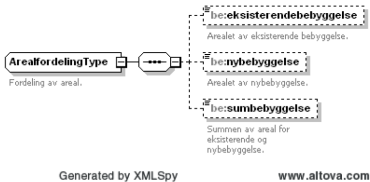
Figure 63 Complex type ArealfordelingType
