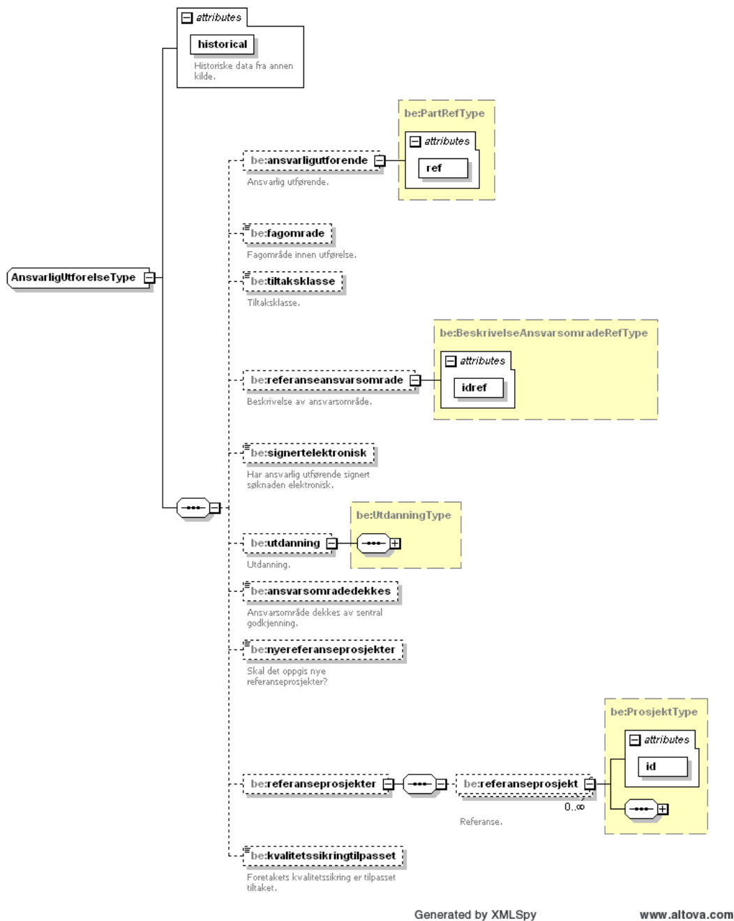
Figure 61 Complex type AnsvarligUtforelseType
