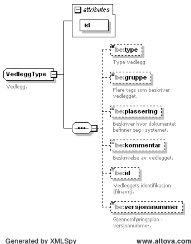
Figure 109 Complex type VedleggType
