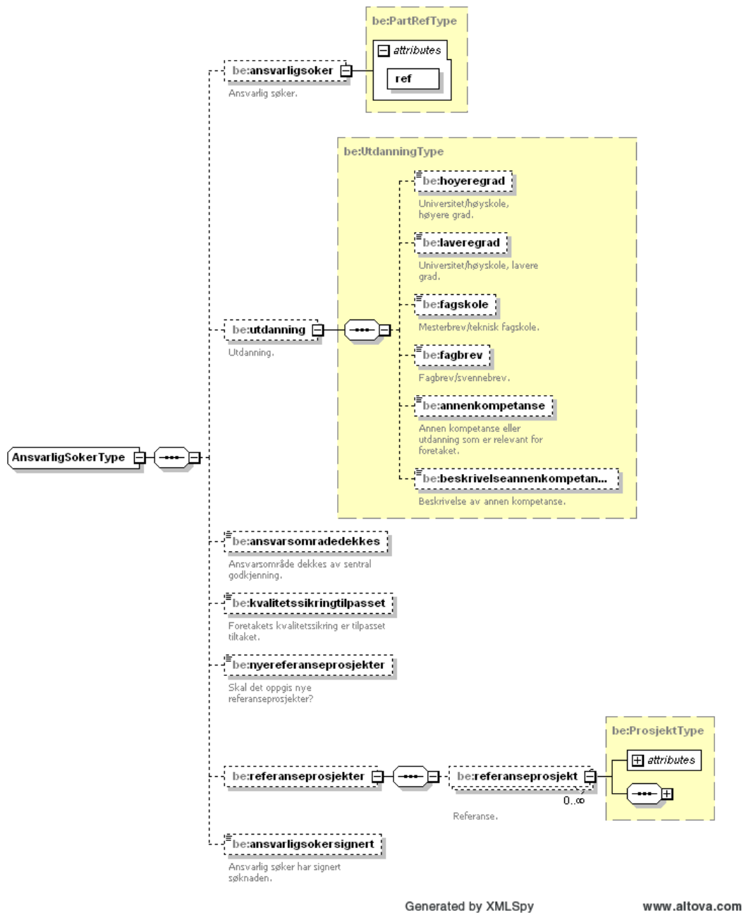
Figure 62 Complex type AnsvarligSokerType
