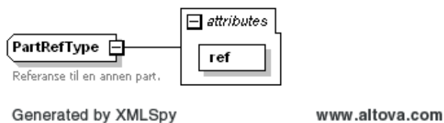
Figure 88 Complex type PartRefType
