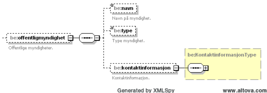
Figure 91 'offentligmyndighet' within PartType
