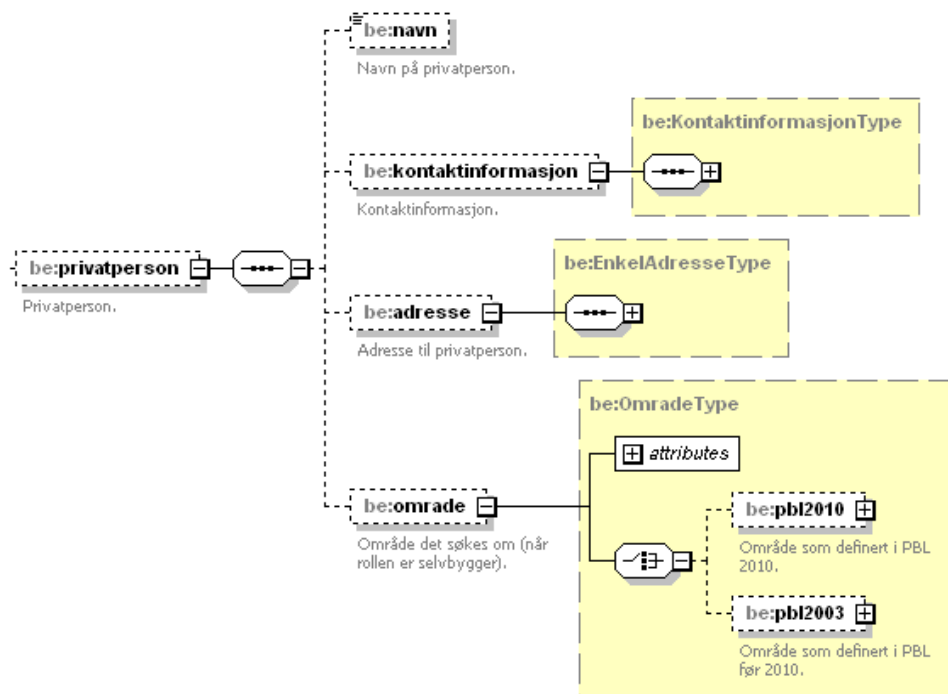
Figure 90 'privatperson' within PartType
