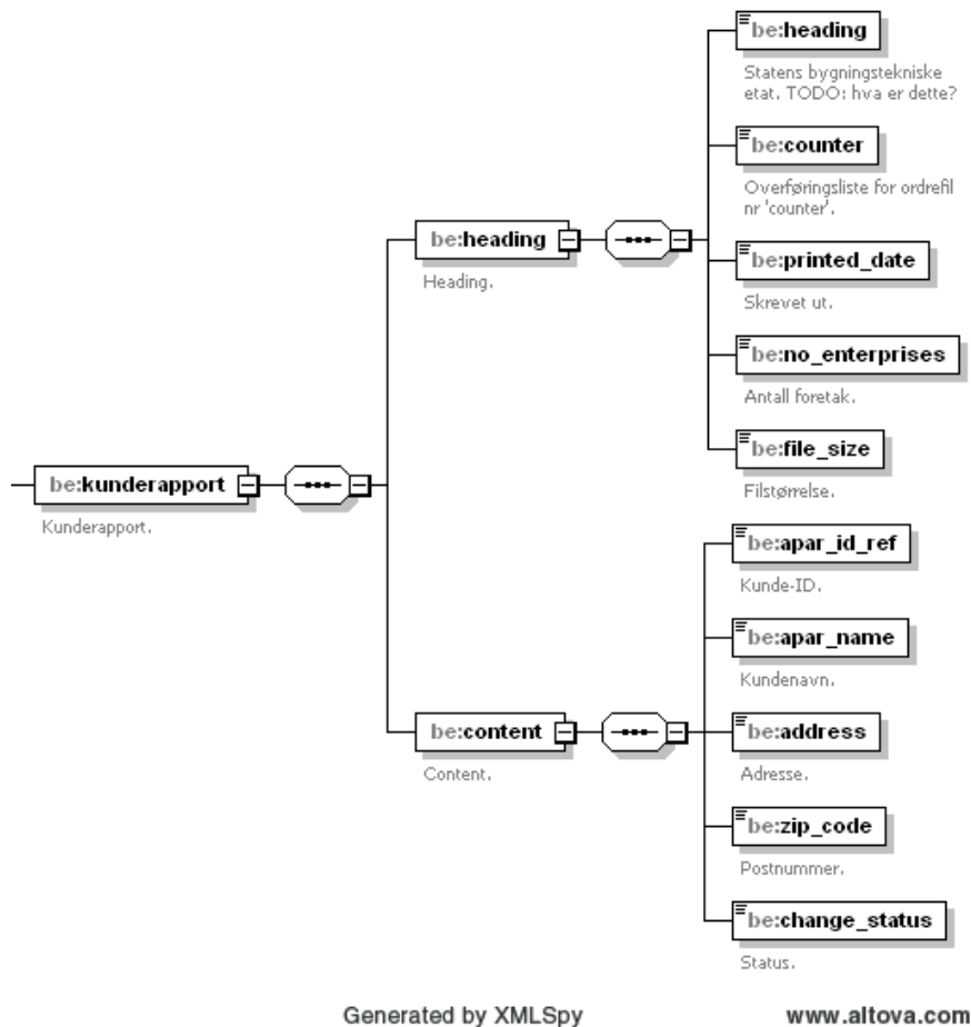
Figure 55 Element structure 'kunderapport' within 'faktura'
