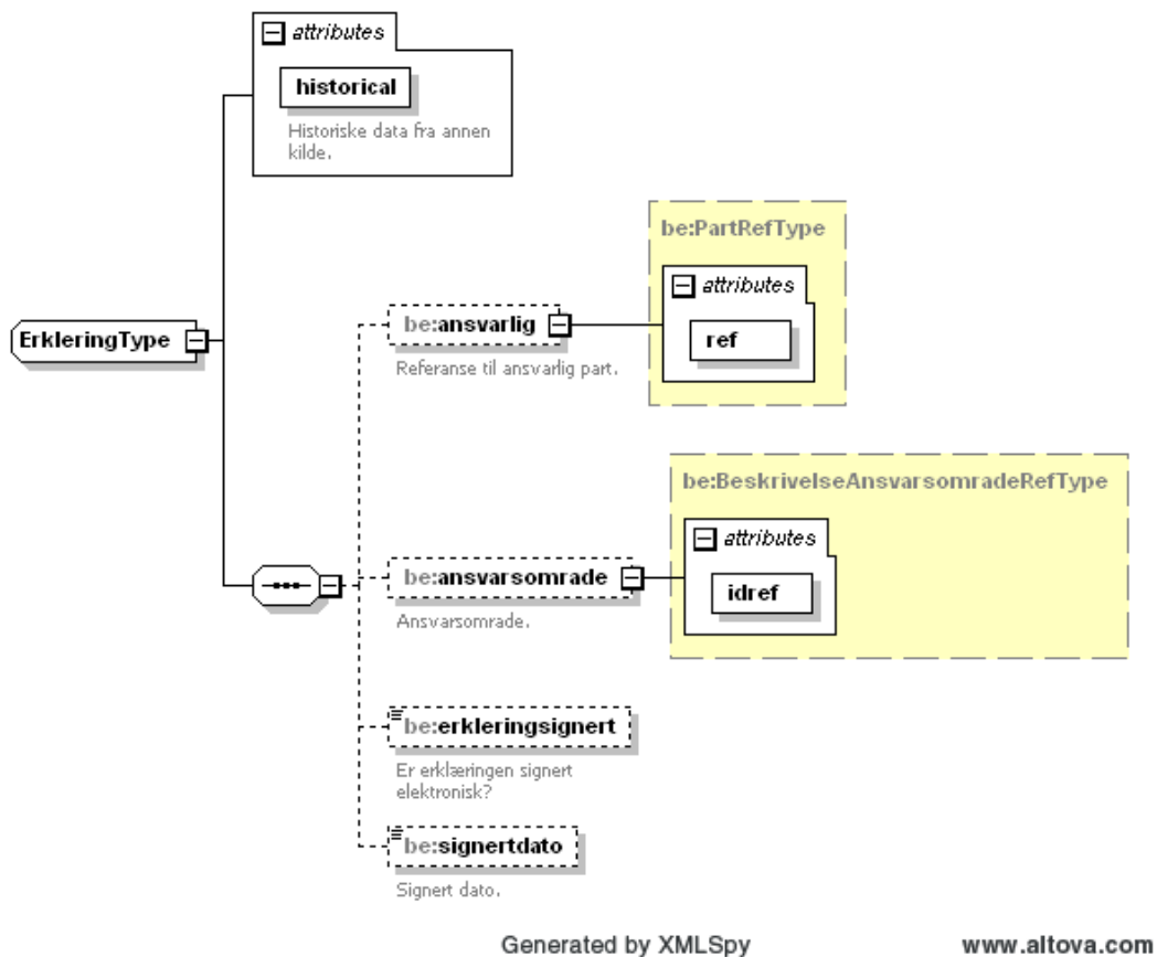
Figure 73 Complex type ErklingType
