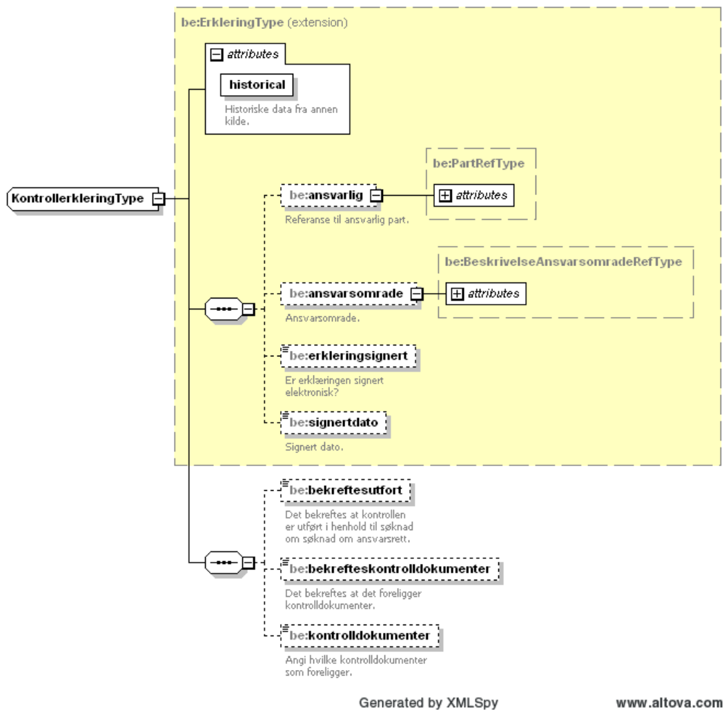
Figure 80 Complex type KontrollerkleringType
