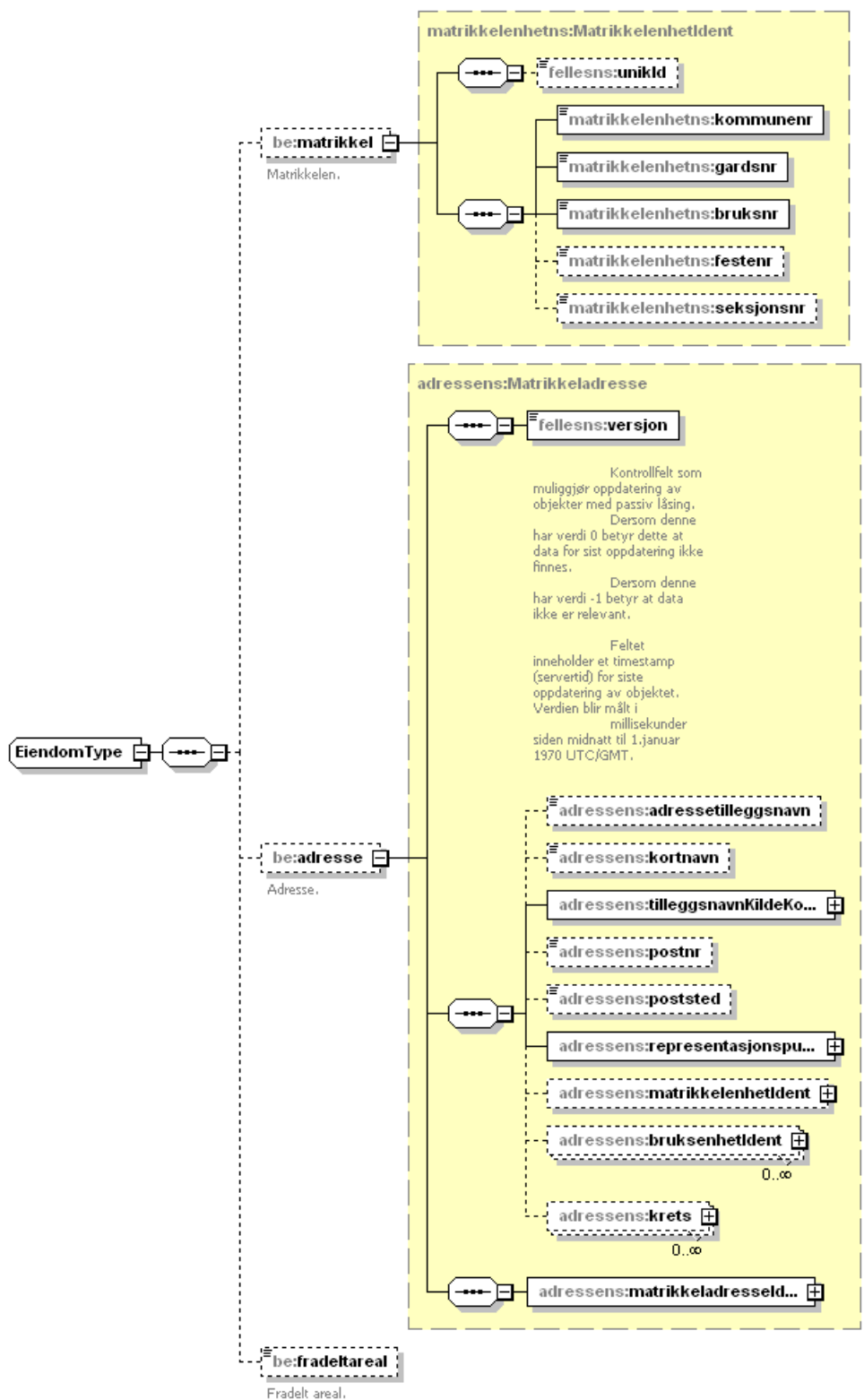
Figure 67 Complex type EiendomType
