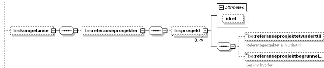
Figure 10 Element structure 'kompetanse' within 'saksbehandling' in 'sentralgodkjenning'
