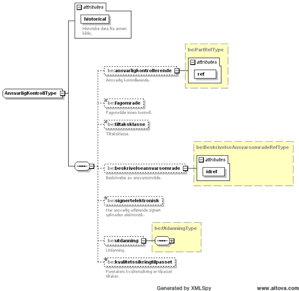
Figure 59 Complex type AnsvarligKontrollType
