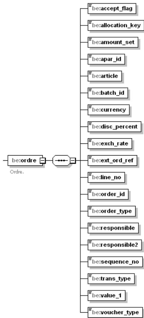
Figure 52 Element structure 'ordre' within 'faktura'
