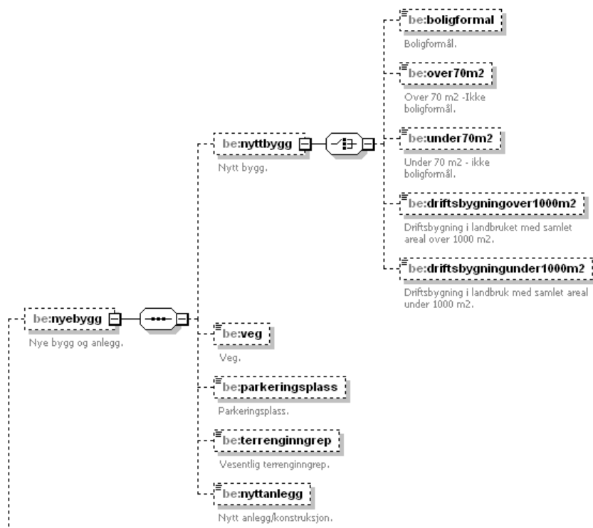
Figure 99 "nyebygg" within TiltakType
