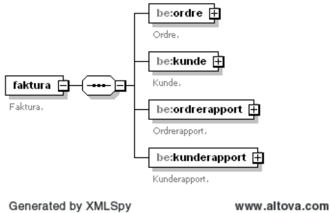
Figure 51 Element structure for 'faktura'
