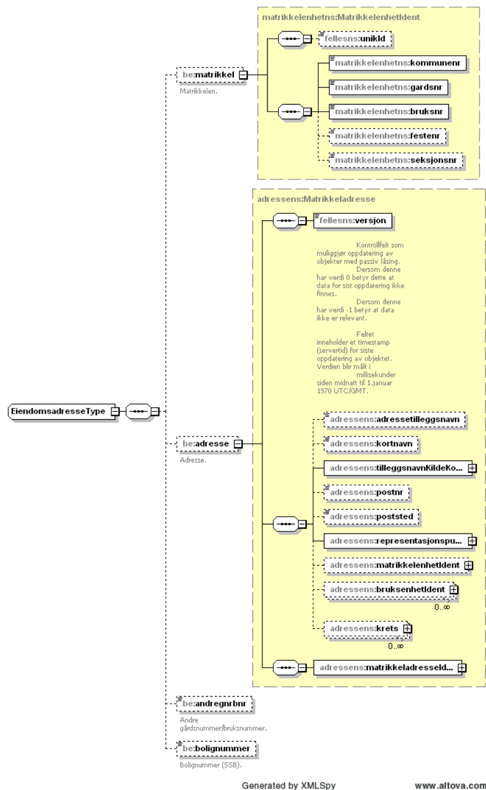
Figure 70 Complex type EiendomsadresseType
