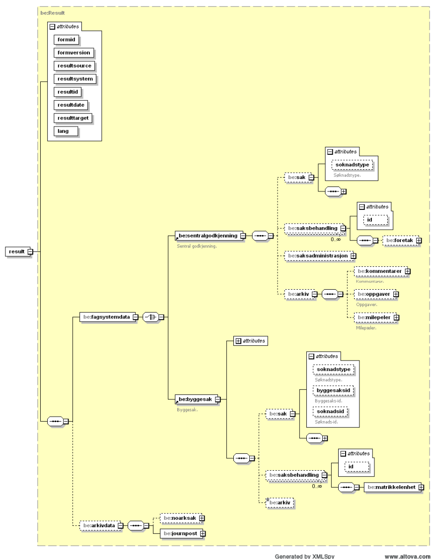
Figure 3 Overview of element structure 'result' of type Result.
