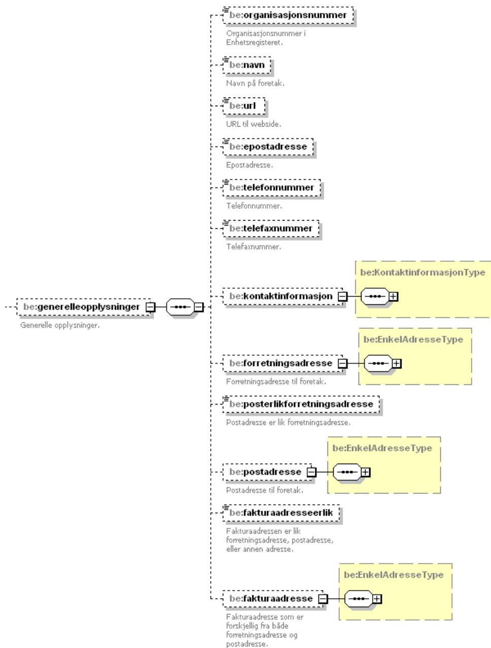
Figure 75 'generelleopplysninger' within ForetakType
