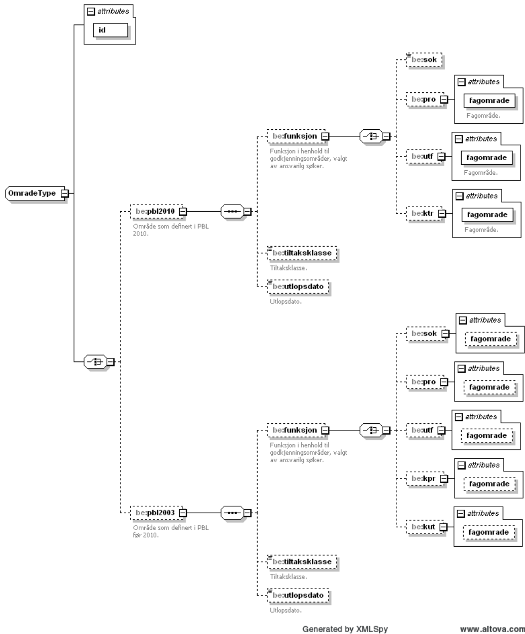
Figure 82 Complex type OmradeType
