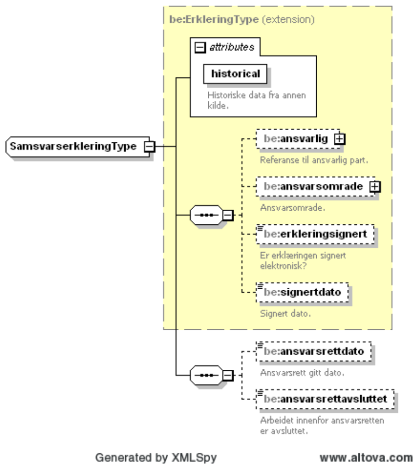
Figure 96 Complex type Samsvarserklæring
