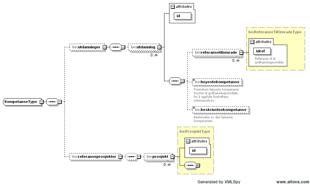
Figure 78 Complex type KompetanseType
