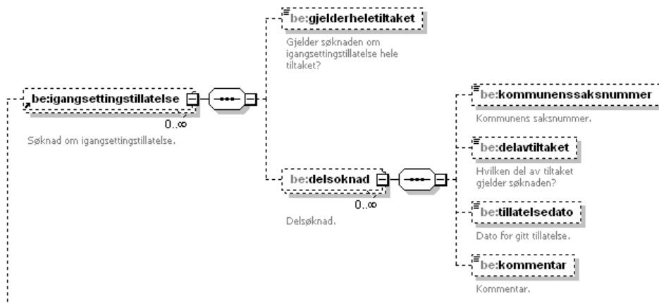
Figure 19 Element structure 'igangsettingstillatelse' within 'soknad' in 'byggesak'
