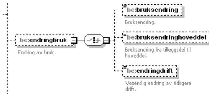
Figure 102 'endringbruk' within TiltakType
