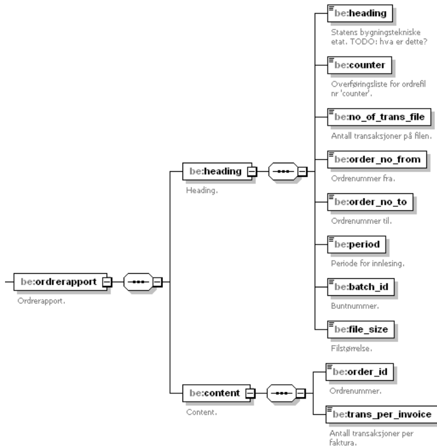
Figure 54 Element structure 'ordrerapport' within 'faktura'
