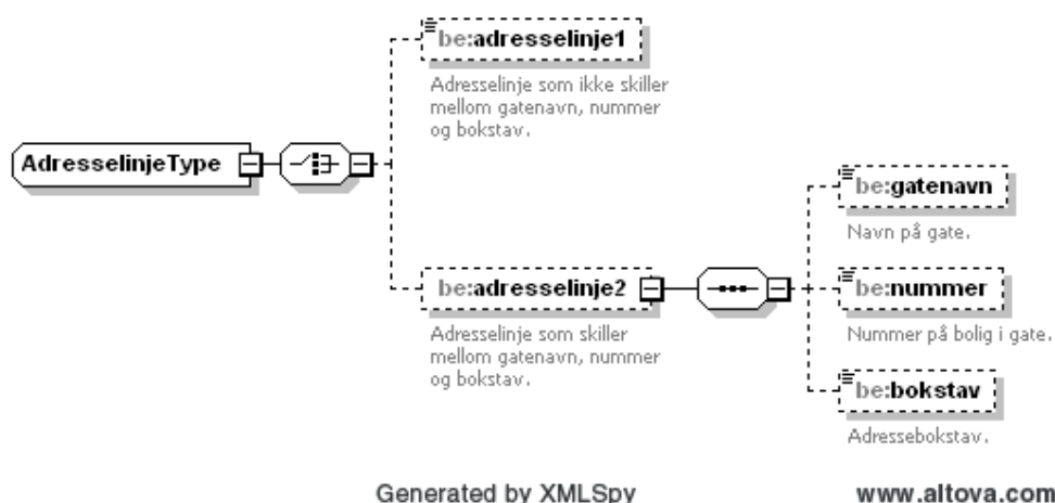
Figure 58 Complex type AdresselinjeType
