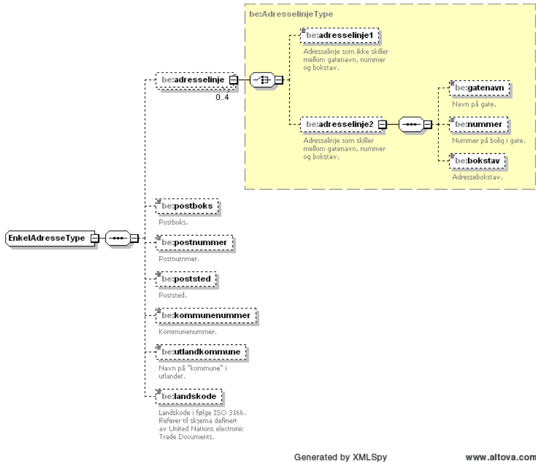
Figure 72 Complex type EnkelAdresseType
