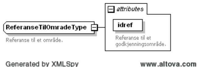
Figure 94 Complex type ReferanseTilOmradeType
