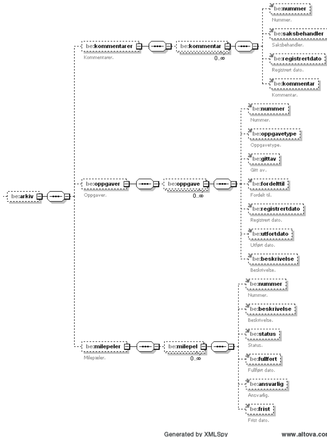
Figure 14 Element structure 'arkiv' within 'sentralgodkjenning'.
