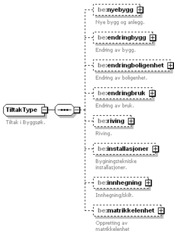
Figure 98 Complex type TiltakType
