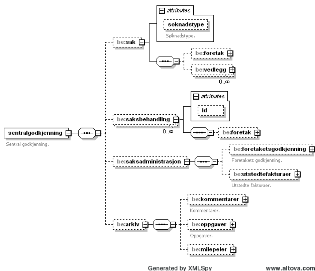
Figure 6 The overall element structure of 'sentral godkjenning'
