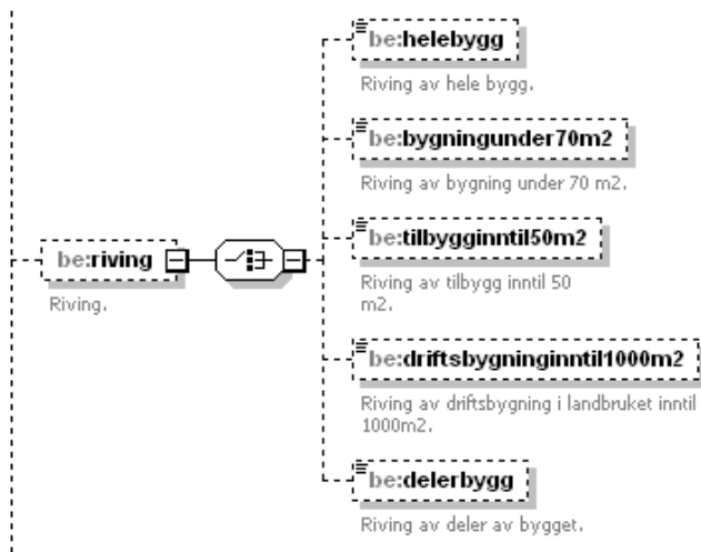
Figure 103 'riving' within TiltakType
