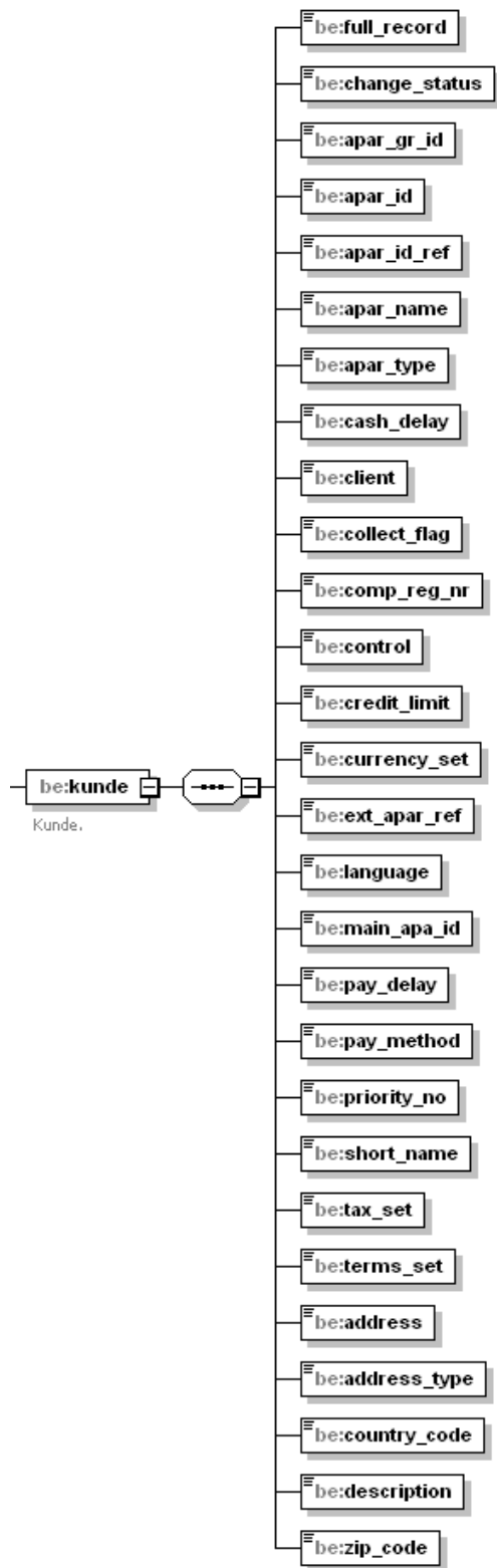
Figure 53 Element structure 'kunde' within 'faktura'
