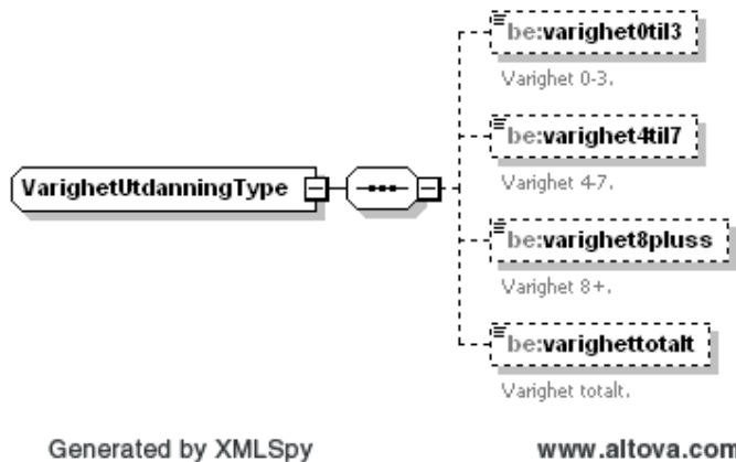
Figure 108 Complex type VarighetUtdanningType
