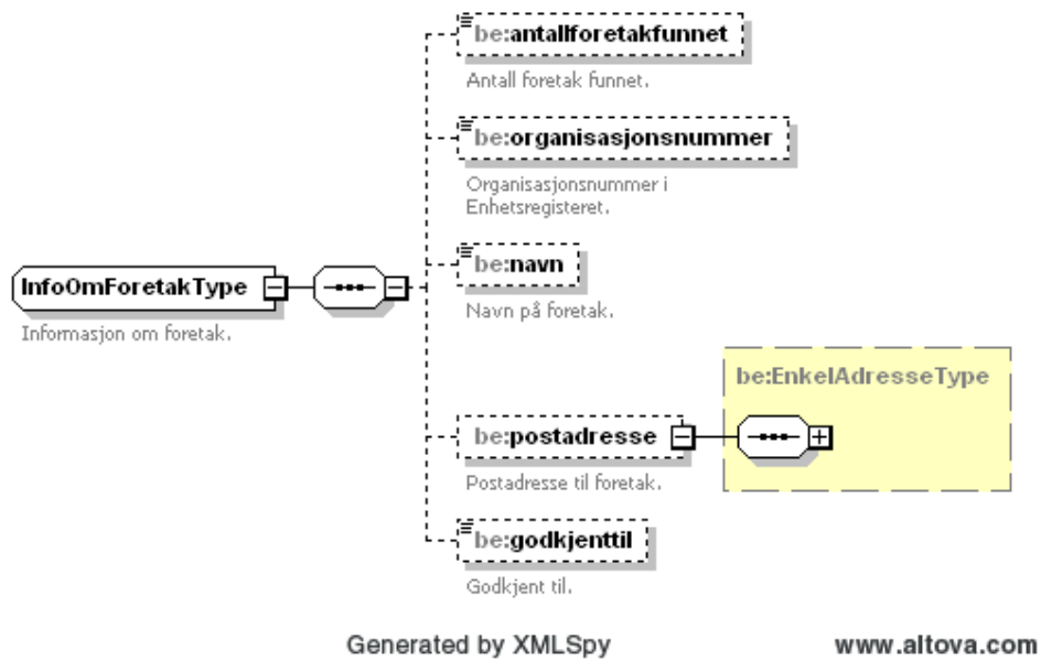
Figure 56 Complex type InfoOmForetakType
