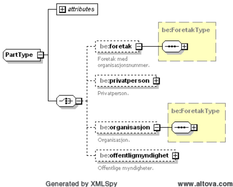
Figure 89 Complex type PartType
