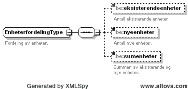
Figure 71 Complex type EnheterfordelingType
